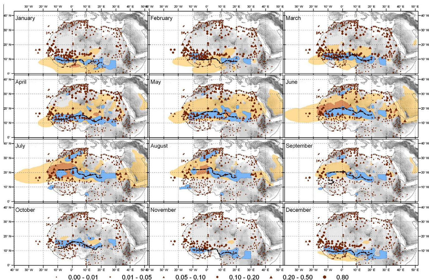
Fig. 4. Relative frequency of dust events over the 26 year period from 1983 to 2008 calculated separately for individual months. The topographic height is shaded in black. The blue areas represent the 8 \times 10^{-6} \text{ s}^{-1} level of horizontal convergence and the black dashed lines the position of the lowest 925 hPa geopotential height between the Equator and 28°N (an indication of the ITD position) as derived by Lavaysse et al. (2009). Yellow and orange areas indicate regions of monthly averaged TOMS/OMI AI exceeding 1.8 and 3 (from Klose et al., 2010).
