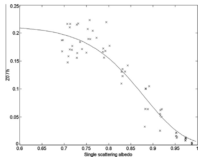
Fig. 16. Model fitted to the single scattering albedo (SSA) of Dong et al. (2002) reconstructed wind tunnel surface roughness and its relationship with the measured aerodynamic roughness length ( z_0 ) standardized by object height ( h ).
