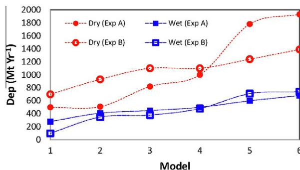
Fig. 14. Inter-comparison of dry and wet depositions for mineral dust as simulated by different global dust models. In Exp-A simulations were done without pre-specifications. In Exp-B simulations were forced with identical dust emission, size distribution and injection height (data from Textor et al., 2006, 2007).
