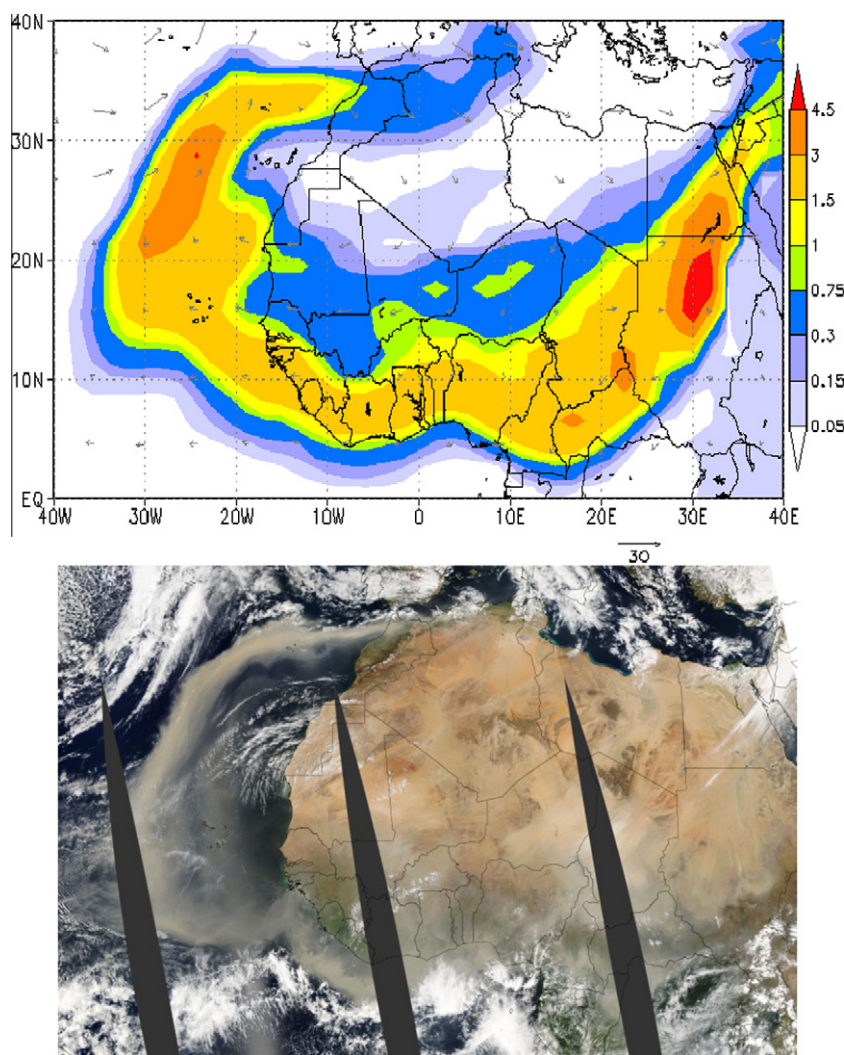
Fig. 12. (a) MASINGAR simulated column dust load in [ \text{g m}^{-2} ] and 700 hPa wind for 12:00UTC 6 March 2004 (Tanaka, 2010 personal communication); (b) Saharan dust storms on 6 March 2004 imaged by MODIS in a series of consecutive overpasses of NASA's Aqua satellite (Image courtesy Jacques Descloitres, MODIS Rapid Response Team, NASA-Goddard Space Flight Center).
