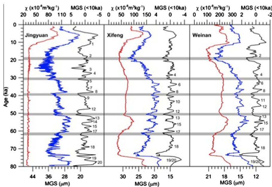
Fig. 11. High resolution grain size variations indicative of monsoon events: magnetic susceptibility ( \chi ), mean grain size (MGS) and high-frequency (<10 kyr) component of the MSG record for three loess sections. Grey bars indicate that coarsening of the MGS can be correlated between the three sections (Sun et al., 2010).
