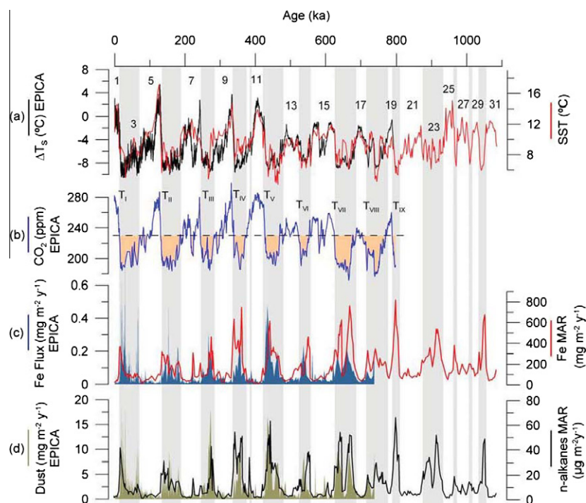
Fig. 9. Marine and terrestrial records over the past 1.1 Ma reconstructed from EPICA ice cores and alkenone data at Site PS2489-2/ODP1090. (a) Temperature from EPICA ice cores (black, Aarctica) and SST from PS2489-2/ODP1090 (red); (b) EPICA CO 2 concentrations. Filled areas illustrate CO 2 concentration below 230 ppmv. (c) EPICA Fe flux (blue) and PS2489-2/ODP1090 Fe flux (red). (d) EPICA insoluble dust (light brown) and PS2489-2/ODP1090 C 23-33 mass accumulation rate (blue). The highest levels of iron (gray vertical bands) correspond to the highest dust concentration, lowest temperature and CO 2 levels in every glacial cycle (for details see Martínez-García et al., 2009).
