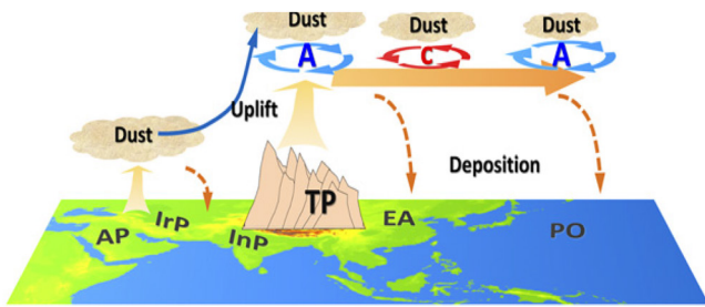
Figure 7. Schematic diagram illustrating dust belt formation during the spring over the Northern Hemisphere. A, anticyclonic circulation center; C, cyclonic circulation center; AP, Arabian Peninsula; IrP, Iranian Plateau; InP, Indian Peninsula; EA, East Asia; PO, Pacific Ocean. Source: C. Xu et al. (2018).
