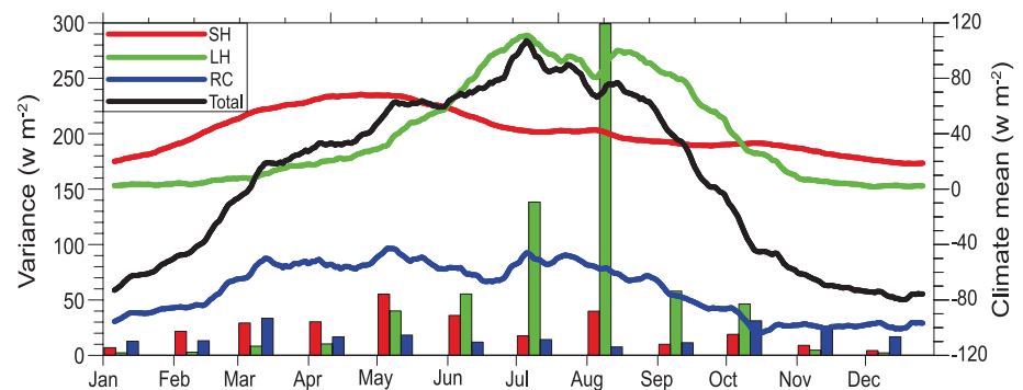
Figure 9. Climatological means (solid lines; \text{W m}^{-2} ) and monthly variance (bars) of each component in the Tibetan Plateau heat source, as determined by averaging data across 73 meteorological observation stations over the TP: Red denotes sensible heating; green is latent heating; blue is net radiation flux of the air column (RC); and black is their sum. Source: Y. Zhao et al. (2018c).
