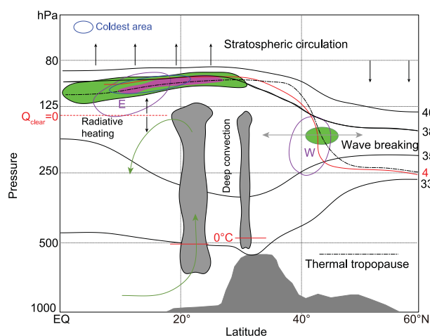
Figure 6. Schematic of the pathways for troposphere-to-stratosphere transport within the Asian summer monsoon anticyclone. At the mean temperature lapse rate tropopause (black dashed line), the density of crossing points is denoted by green and purple shadings, depicting lower, and higher densities, respectively. The coldest region (blue circle) is overlaid on the color-shaded area. Vertical motion in the upper troposphere and lower stratosphere is denoted by solid black vertical arrows; whereas the neutral radiative heating level on the tropical side is denoted by a dashed red line, and the isentropic surfaces from 330 to 400 K are represented by solid black lines. The 4-potential vorticity unit is depicted as a solid red line, while the stratosphere–troposphere exchange due to eddy shedding to the north of the anticyclone is denoted by the gray arrows along the isentropic surface. Deep monsoon convections are displayed as the two Gy cloud towers: one for bulky convection over South Asia, and the other for thinner convection over the Tibetan Plateau; whereas the freezing levels are displayed by solid red lines. The vertical monsoon circulation is denoted by green arrows, while the westerly and easterly jets in the upper troposphere are denoted as pink circles. Source: Bian et al. (2020).
