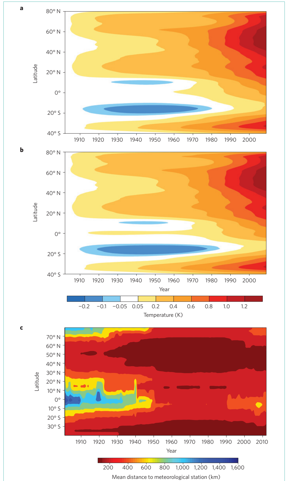
Figure 1 | Temporal evolution of the zonally averaged trend of surface air temperature and of zonally averaged spatial coverage of data. a , Fig. 3 of Ji et al. 4 showing the temporal evolution of the zonally averaged trend of surface air temperature. b , Same as panel a but with the low-standard-deviation areas removed in the averaging process. Note that the colour intervals are uneven. c , Supplementary Fig. 2 of Macias-Fauria et al. 1 showing the temporal evolution of the zonally averaged minimum distance to a meteorological station.
