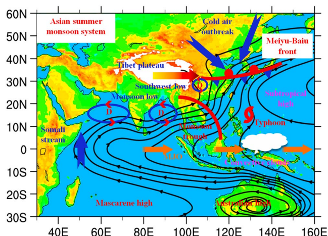
Figure 2. A schematic of the dominant major large-scale low-level moisture transport pathways and weather systems over the Asia-West Pacific region. Colored arrows show the movement of air associated with a given weather system like low-pressure systems (denoted by “D”) or atmospheric phenomenon like the Madden-Julian Oscillation (MJO).
