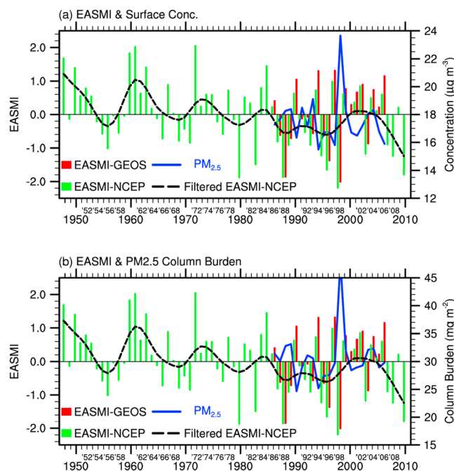
Figure 28. (a) The normalized time series of the EASM index (EASMI, bars, left y axis, [Li and Zeng, 2002; J. P. Li et al., 2010]) and simulated JJA surface layer PM 2.5 concentrations (blue line, right y axis, \mu\text{g m}^{-3} ) averaged over eastern China (110°–125°E, 20°–45°N) for the years 1986–2006. The EASMI-GEOS for the years 1986–2006 (red bars) are calculated using GEOS-4 assimilated meteorological data, while the EASMI-NCEP for the years 1948–2010 (green bars) are calculated using the NCEP/NCAR reanalysis data. The thick dashed line is the 9 year Gaussian-type filtered value of the EASMI-NCEP, which represents the decadal variation in EASM. (b) The same as Figure 28a but for tropospheric column burdens of PM 2.5 (right y axis, \text{mg m}^{-2} ). Copied from Zhu et al. [2012].
