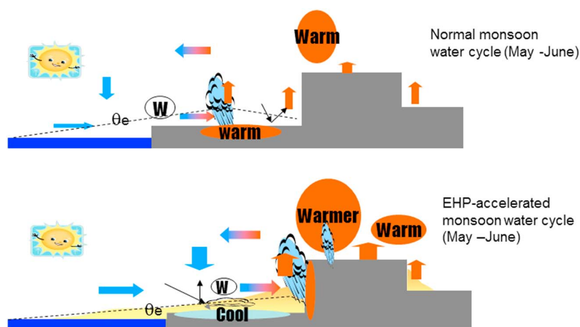
Figure 24. Diagram illustrating the elevated heat pump (EHP) hypothesis. Schematic showing the monsoon water cycle (top) with no aerosol forcing and (bottom) with the aerosol-induced EHP effect. Low-level monsoon westerlies are denoted by W. The dashed line indicates magnitude of the low-level equivalent potential temperature \theta_e . Deep convection is indicated over regions of maximum \theta_e . Arrows denote air circulation. Copied from Lau et al. [2008]. ©American Meteorological Society. Used with permission.
