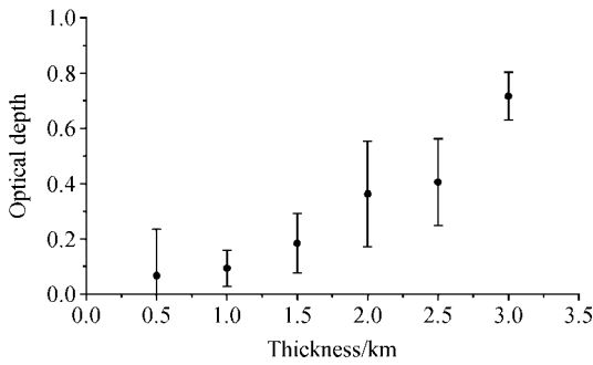
图 11 卷云光学厚度与卷云厚度相关关系 Fig. 11 Cirrus cloud optical depth as a function of cirrus cloud thickness
