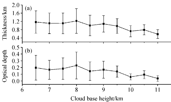
图 12 卷云 (a) 厚度和 (b) 光学厚度随云底高度的变化特征 Fig. 12 (a) Thickness and (b) optical depth of cirrus cloud as a function of cloud base height
