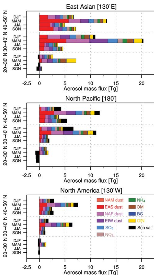
Figure 9. Meridional variations of East Asian outflow across the North Pacific and North American inflow of aerosol seasonal mass flux for 2010–2014.
