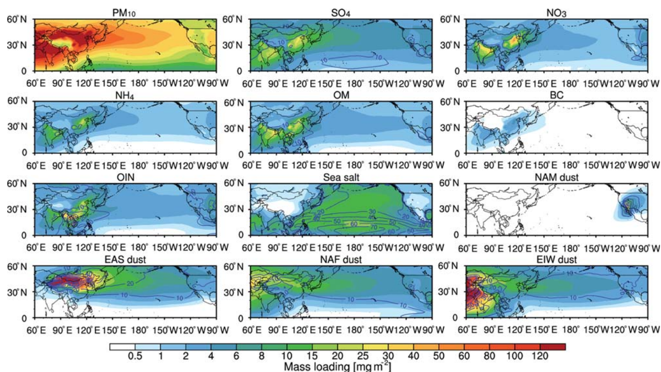
Figure 3. Spatial distribution of aerosol composition column mass loading from WRF-Chem averaged for 2010–2014. The trans-Pacific transport aerosol mass spatial distribution is denoted by \text{PM}_{10} and the dust from North America, East Asia, north Africa, and elsewhere in the world is denoted by NAM dust, EAS dust, NAF dust, and EIW dust. Contour lines (blue solid line) denote the percentage contribution (%) of the corresponding aerosol composition to total aerosol column mass.
