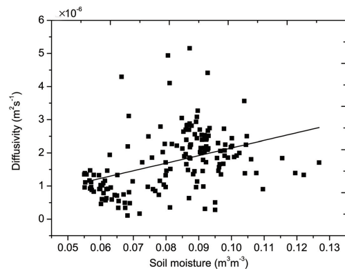
Fig. 10. Relationship between soil moisture and soil thermal diffusivity in the dry season.
