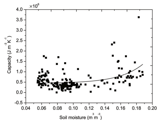
Fig. 9. Relationship between soil moisture and soil heat capacity in the dry season.
