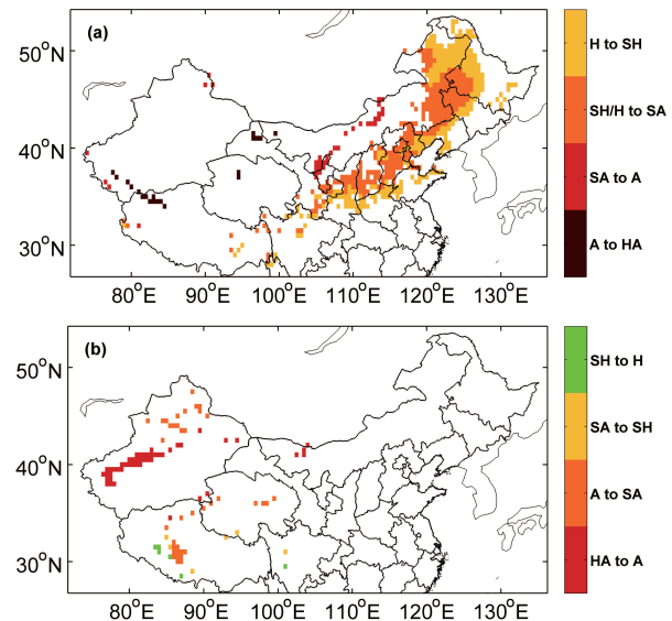
Fig. 4. Changes in coverage to (a) drier types and (b) wetter types for 1994–2008 relative to 1961–90. H, SH, SA, A, and HA represent humid, subhumid, semi-arid, arid and hyper-arid, respectively.
