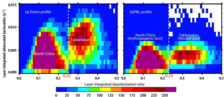
Figure 3. The relationship between the layer-integrated depolarization ratio and the layer-integrated attenuated backscatter coefficient for anthropogenic dust (North China) and natural dust (Taklamakan) for (a) the entire profile, and (b) the PBL profile.
