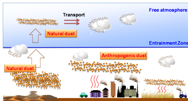
Figure 2. A schematic figure for the detection process of anthropogenic dust.
