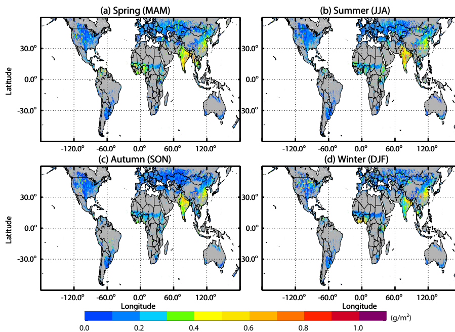
Figure 6. Global seasonal distributions of mean anthropogenic dust column burden (2007–2010) for spring–winter, (a)–(d), respectively. The gray areas represent non-anthropogenic dust source over land.
