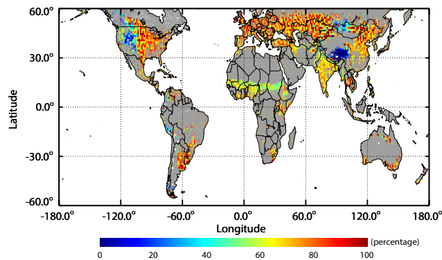
Figure 7. Global distributions of the percentage of anthropogenic dust column burden account for total dust column burden.
