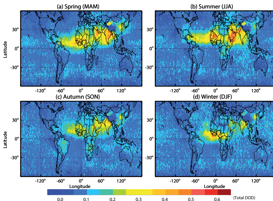
Figure 5. Global seasonal distributions of total (including polluted dust) dust optical depth derived from CALIPSO measurements (2007–2010) for spring–winter, (a)–(d), respectively.
