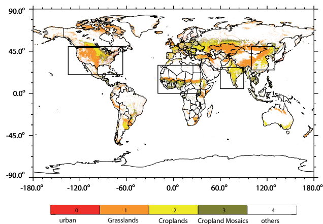
Figure 1. Global anthropogenic land cover (including urban, cropland, and pastureland) distribution retrieved by combining MODIS and GRUMP data.
