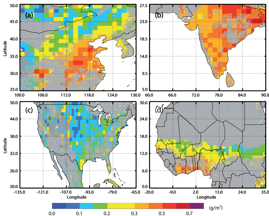
Figure 9. Regional distribution of annual mean anthropogenic dust column burden derived from CALIPSO measurements (2007 through 2010) for (a) eastern China, (b) India, (c) North America, and (d) North Africa.
