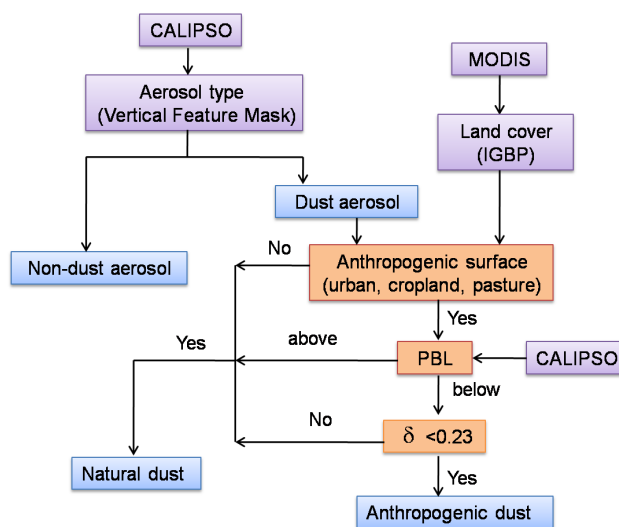
Figure 4. Flow chart of anthropogenic dust detection by combing CALIPSO and land cover data set provided by MODIS.
