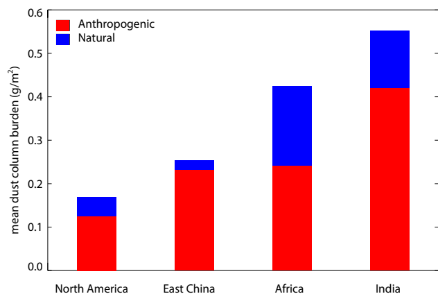
Figure 10. Anthropogenic (red) and natural (blue) mean dust column burdens and percentages in four regions (eastern China, India, North America and Africa).
