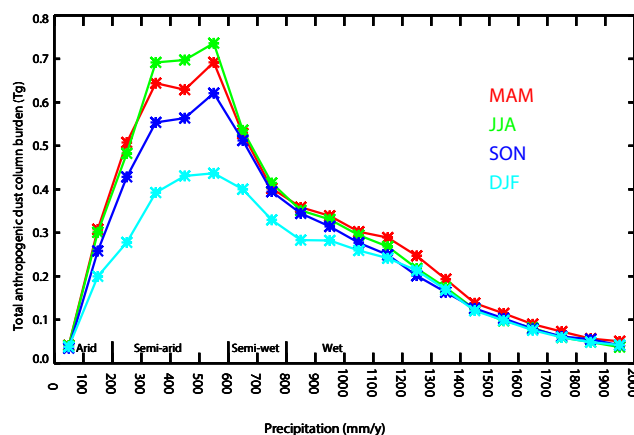
Figure 8. Comparisons of dust column burden as function of climatological mean precipitation for different four seasons (spring, summer, autumn, and winter) of global anthropogenic land cover. The precipitation interval is 100 mm yr -1 .
