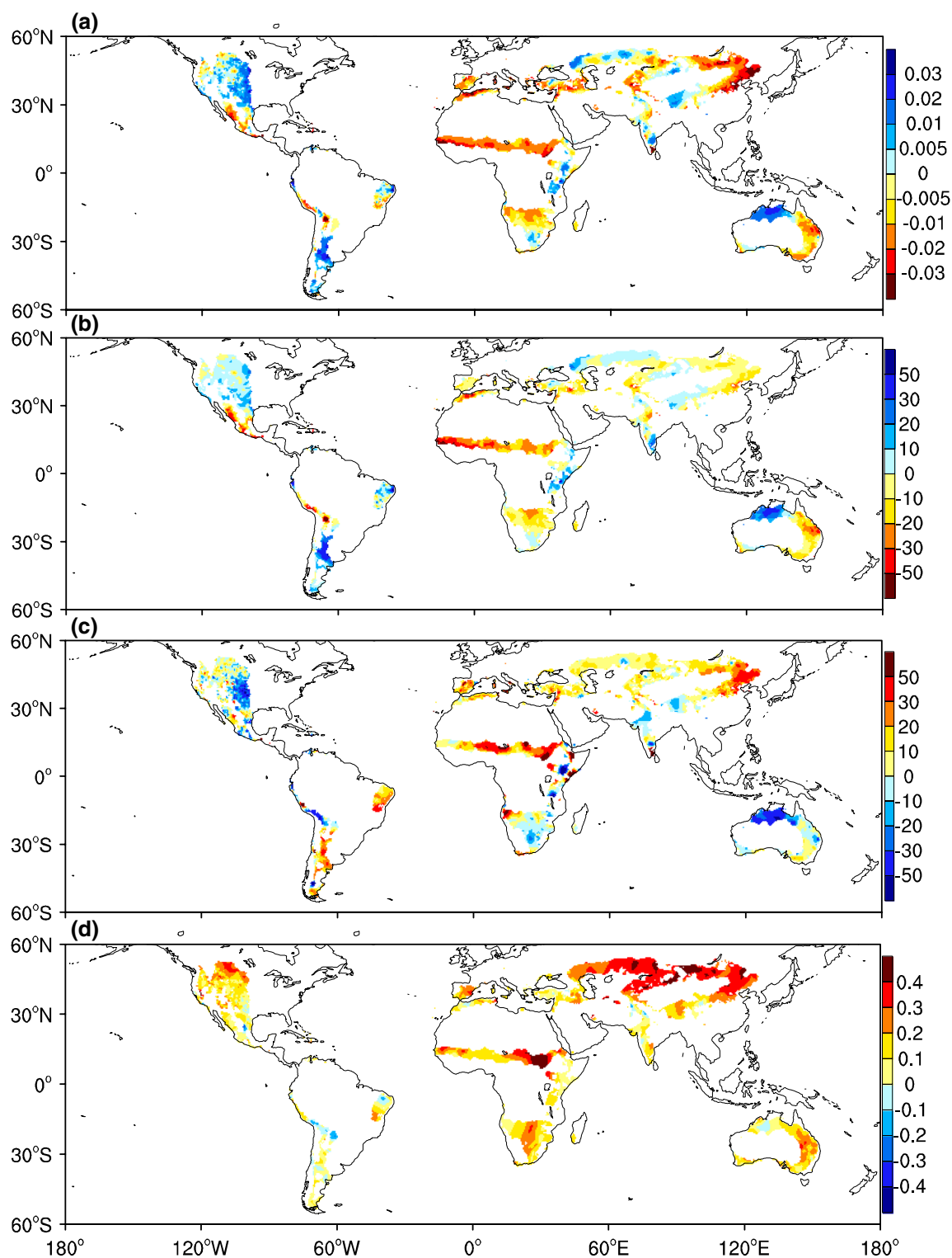
Fig. 5 The distributions of the linear trends in the AI, precipitation, PET, and SAT in semi-arid regions globally from 1948 to 2008. a P/PET trend (/decade), b P trend (mm/decade), c PET trend (mm/decade), d temperature trend (°C/decade)
